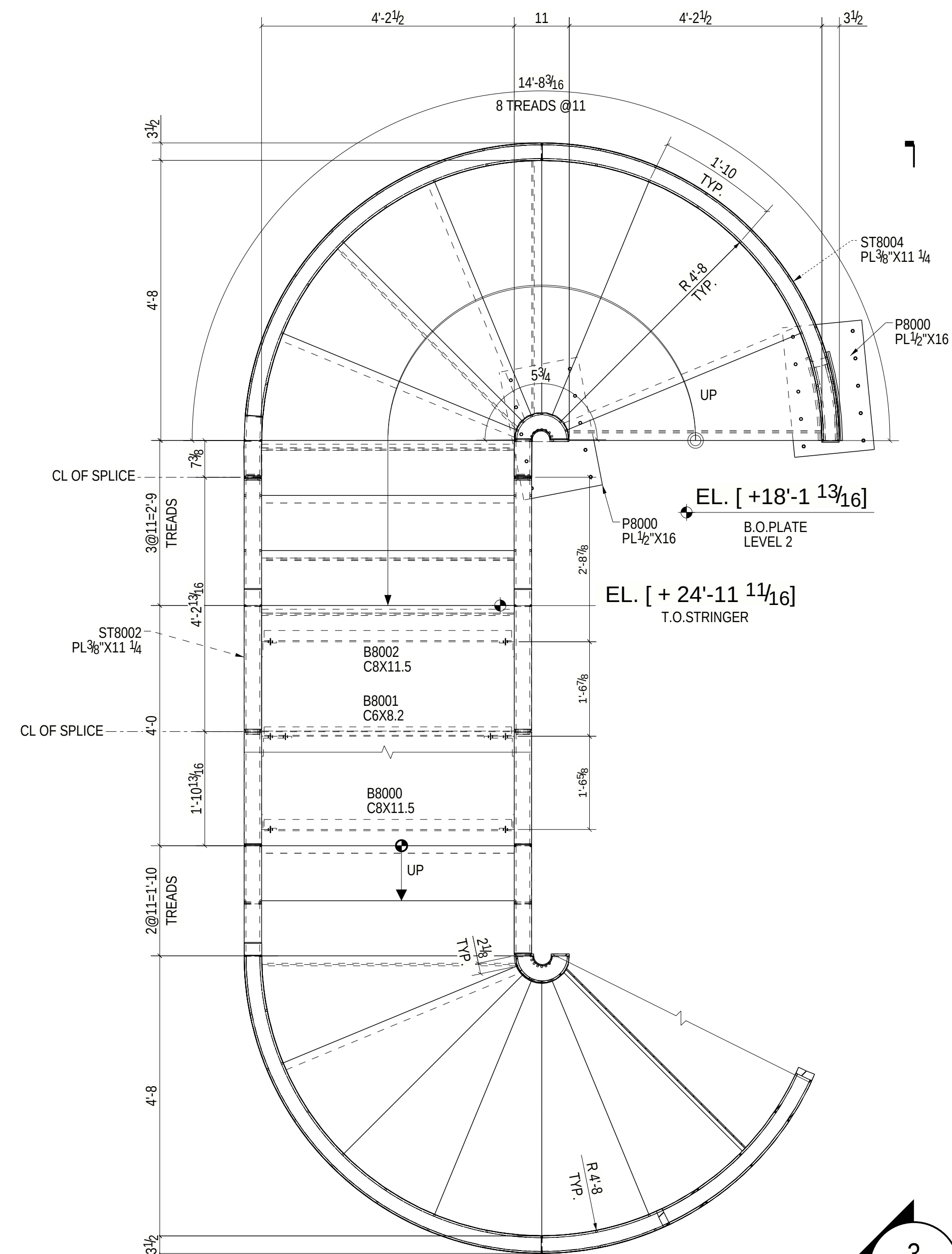
1 STAIR PLAN @ LEVEL 2
