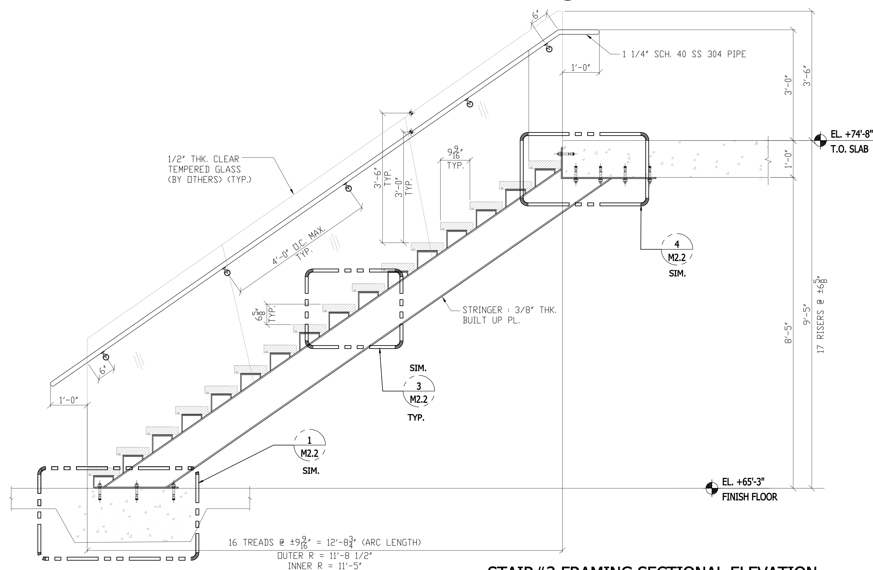
2 STAIR#3 FRAMING SECTIONAL ELEVATION
