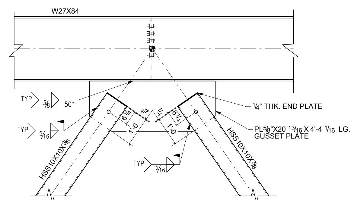
2 DETAIL VIEW SCALE: 1:24
