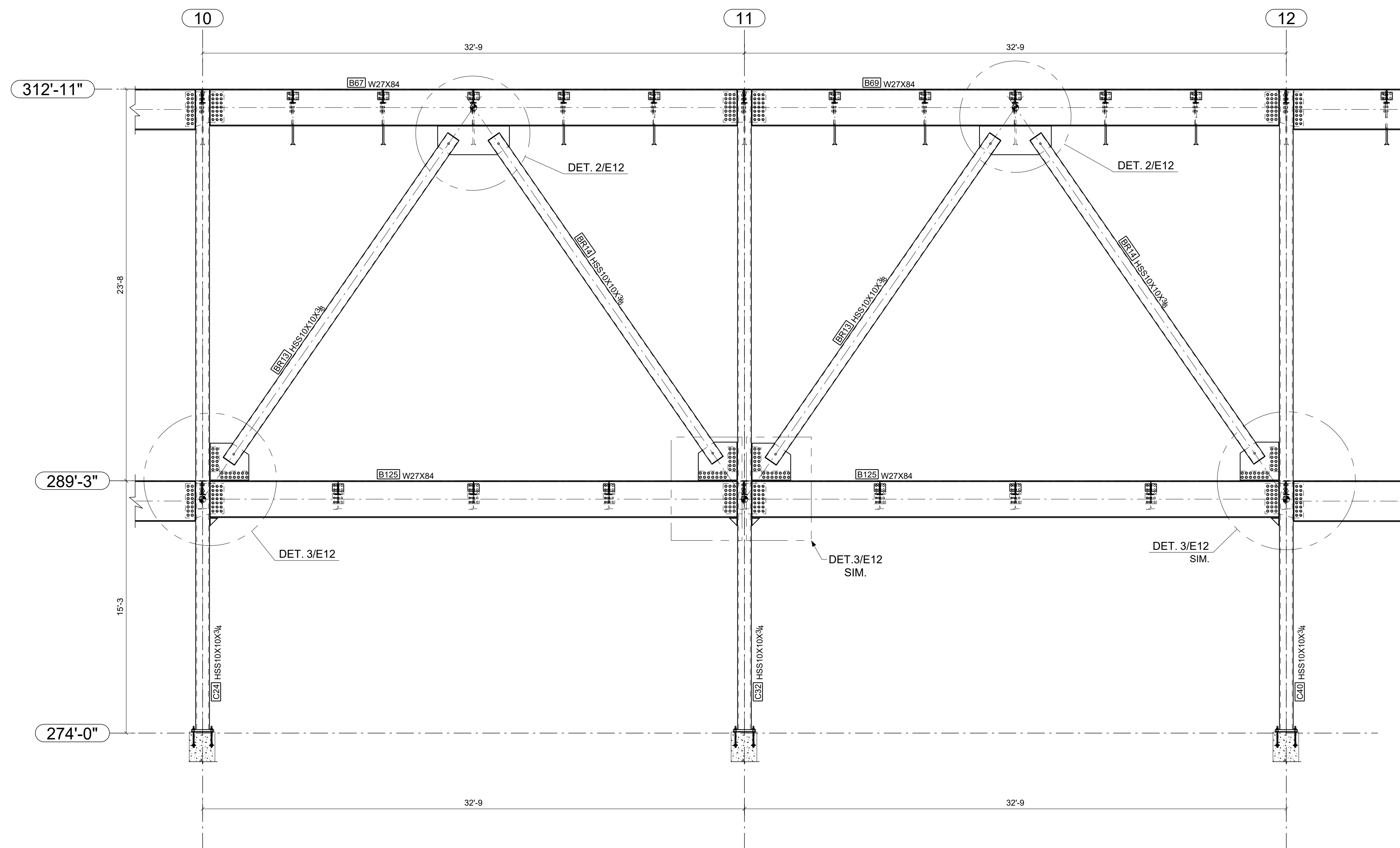
1 BRACE ELEVATION ALONG GRID LINE D-4 SCALE: 1:48
