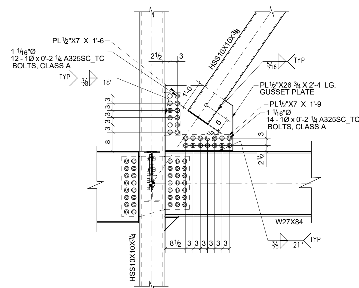
3 DETAIL VIEW SCALE: 1:24
