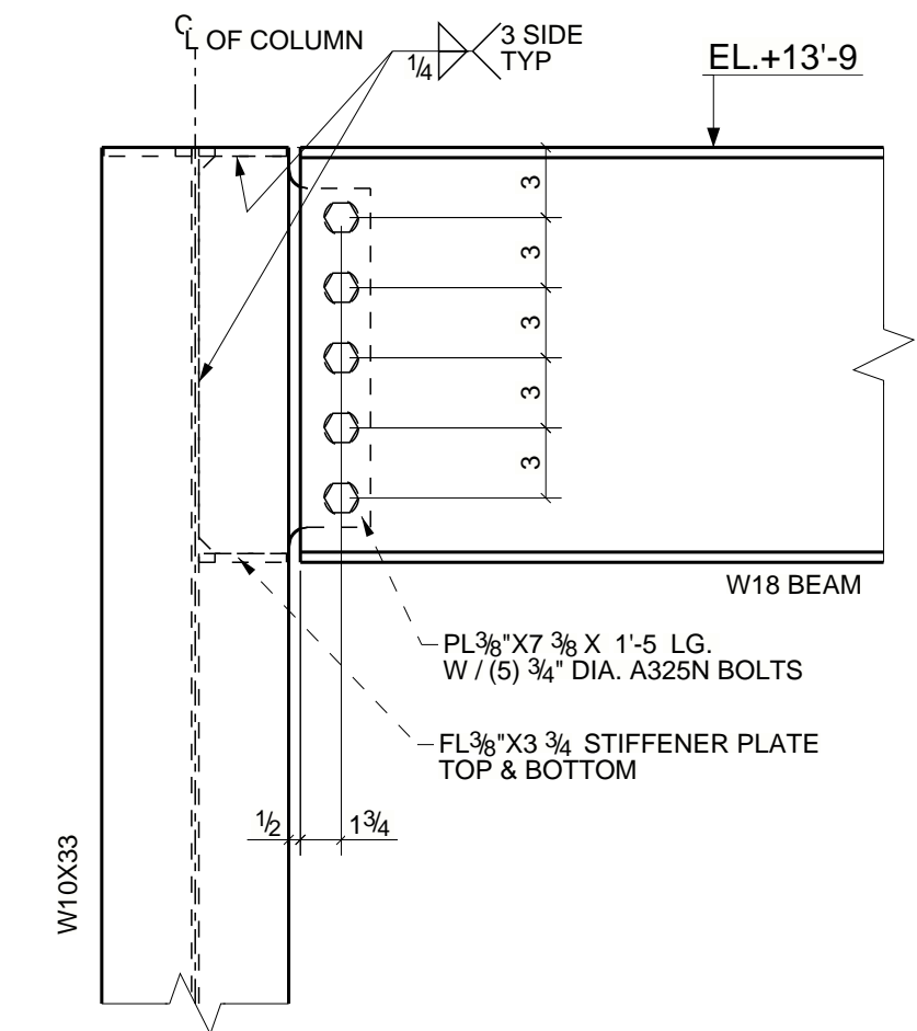
W18 BEAM TO W10 COLUMN
