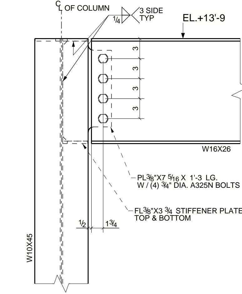
W16 BEAM TO W10 COLUMN
