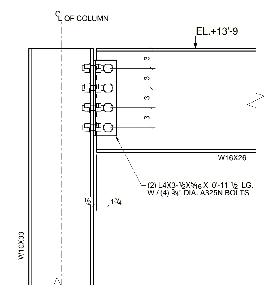
W16X26 BEAM TO W10 COLUMN
