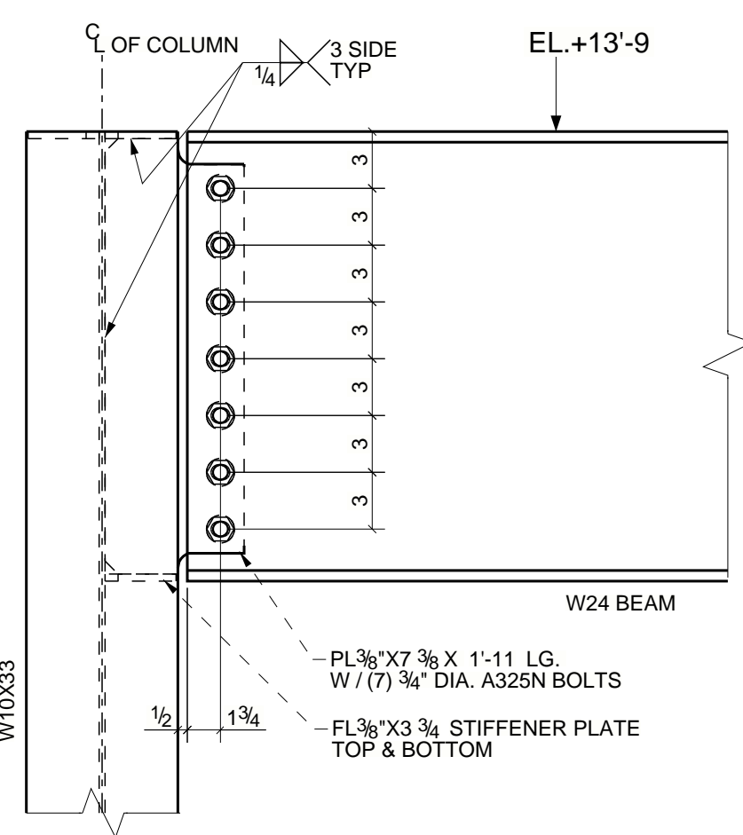
W24 BEAM TO W10 COLUMN
