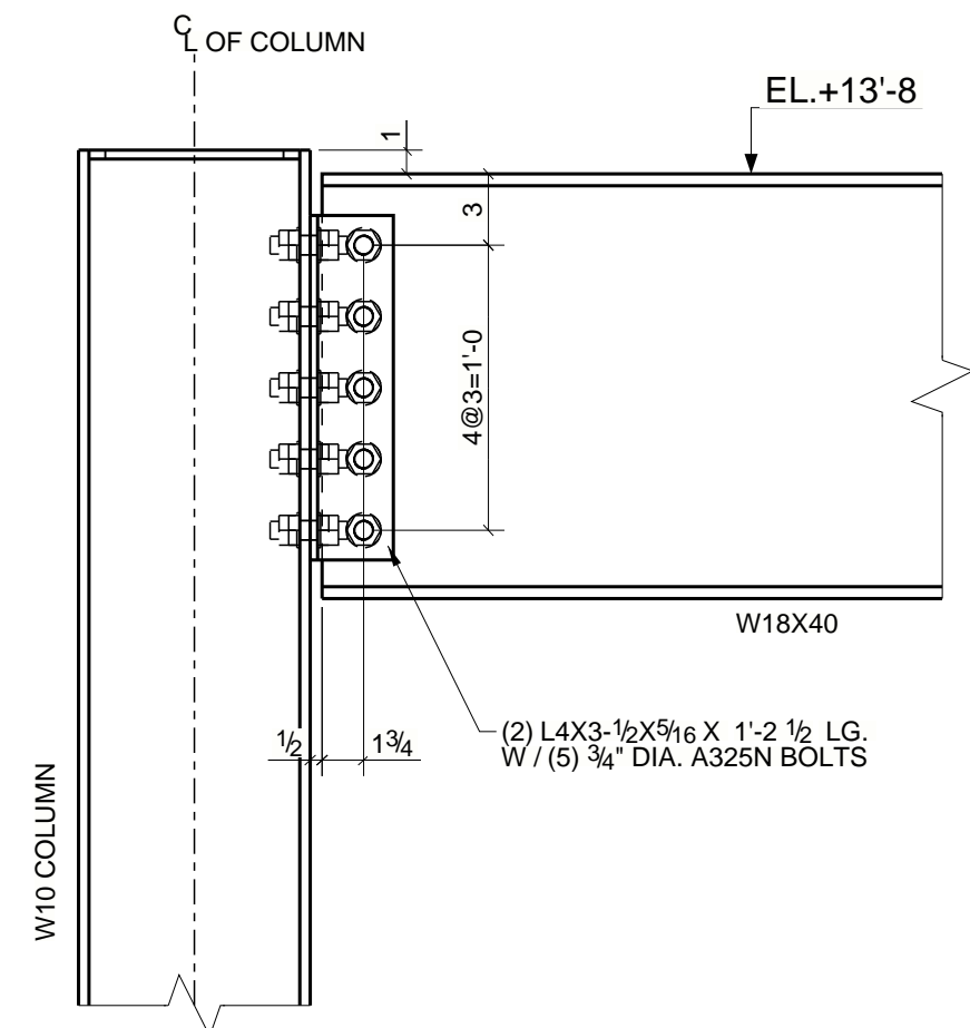
W18X40 BEAM TO W10 COLUMN
