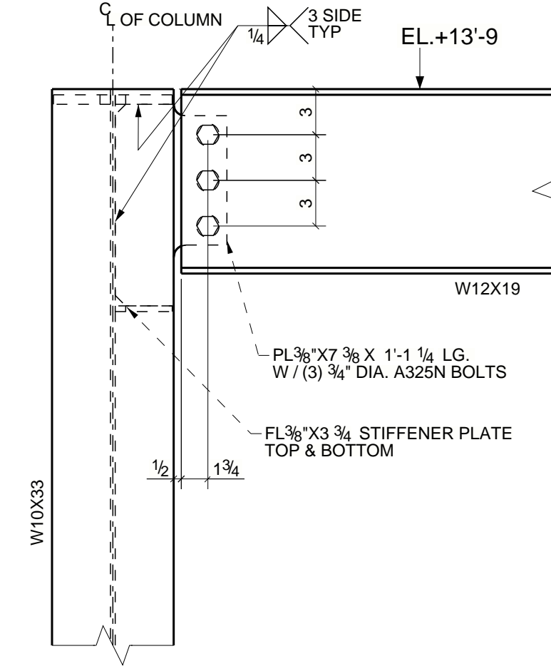
W12 BEAM TO W10 COLUMN
