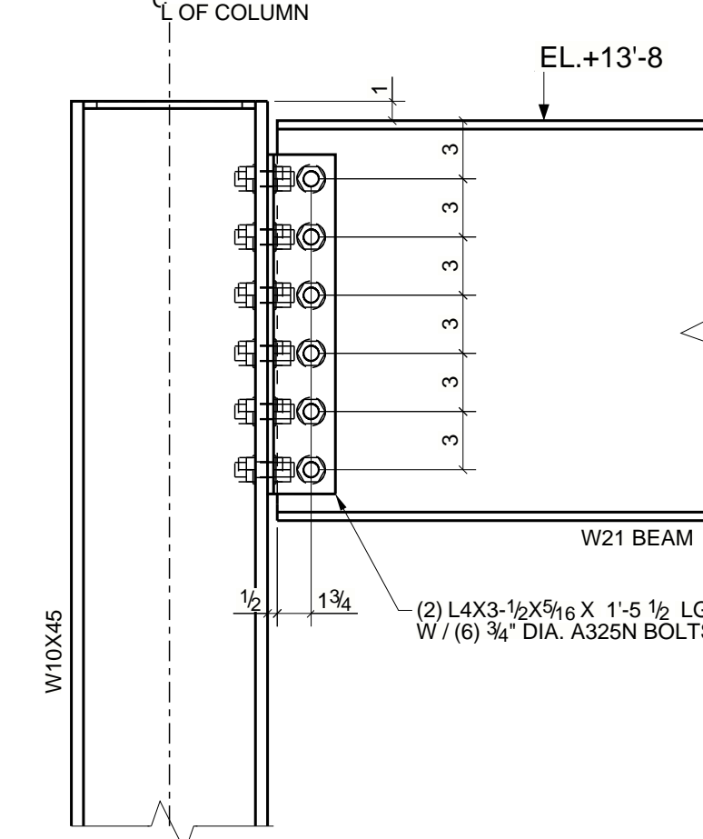
W21 BEAM TO W10 COLUMN
