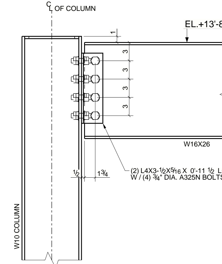
W16X26 BEAM TO W10 COLUMN
