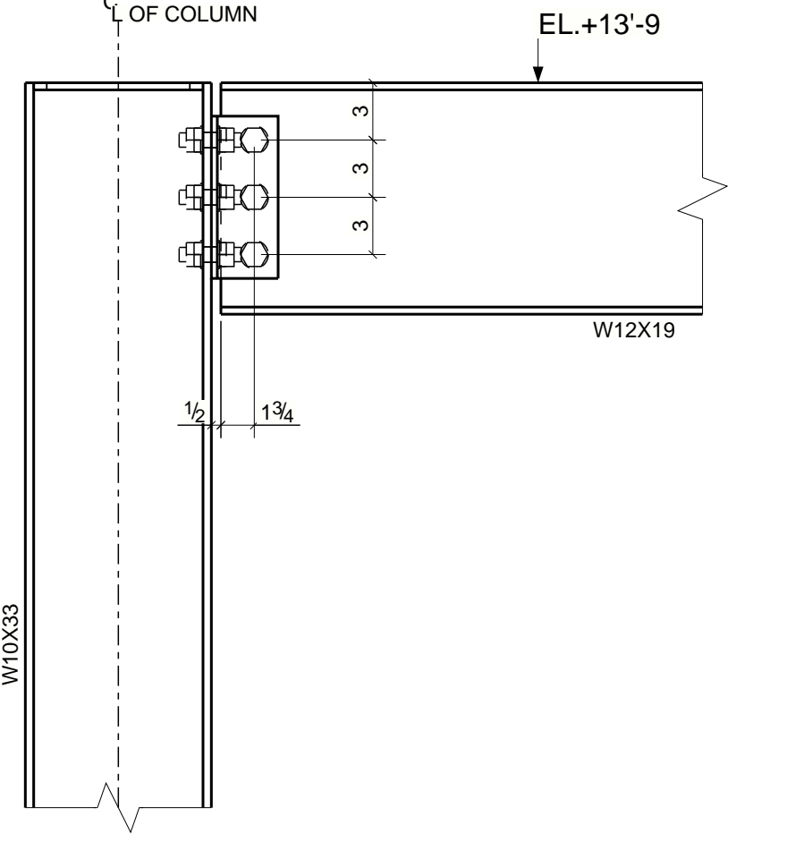
W12X19 BEAM TO W10 COLUMN
