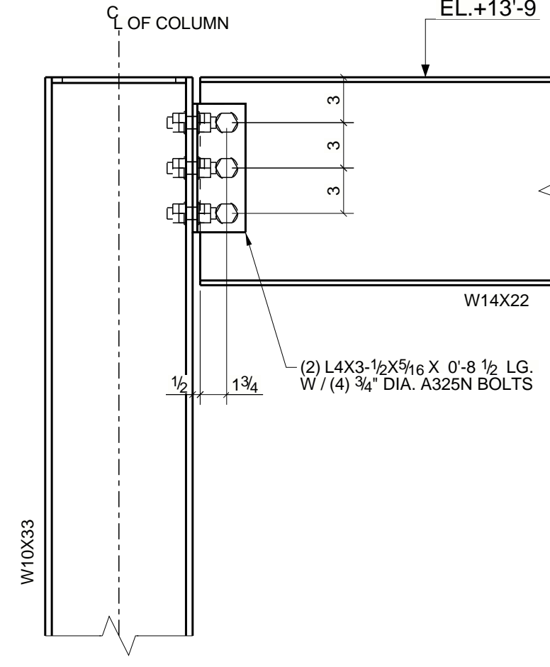
W14 BEAM TO W10 COLUMN
