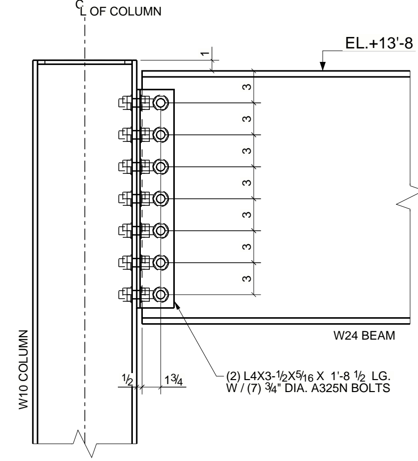
W24 BEAM TO W10 COLUMN
