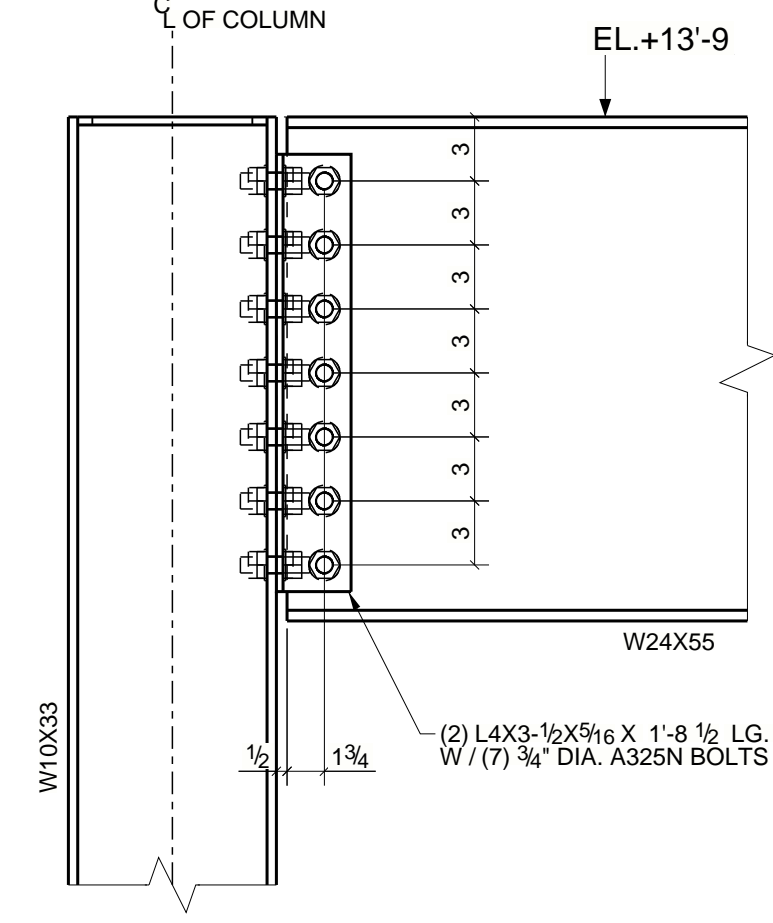
W24 BEAM TO W10 COLUMN
