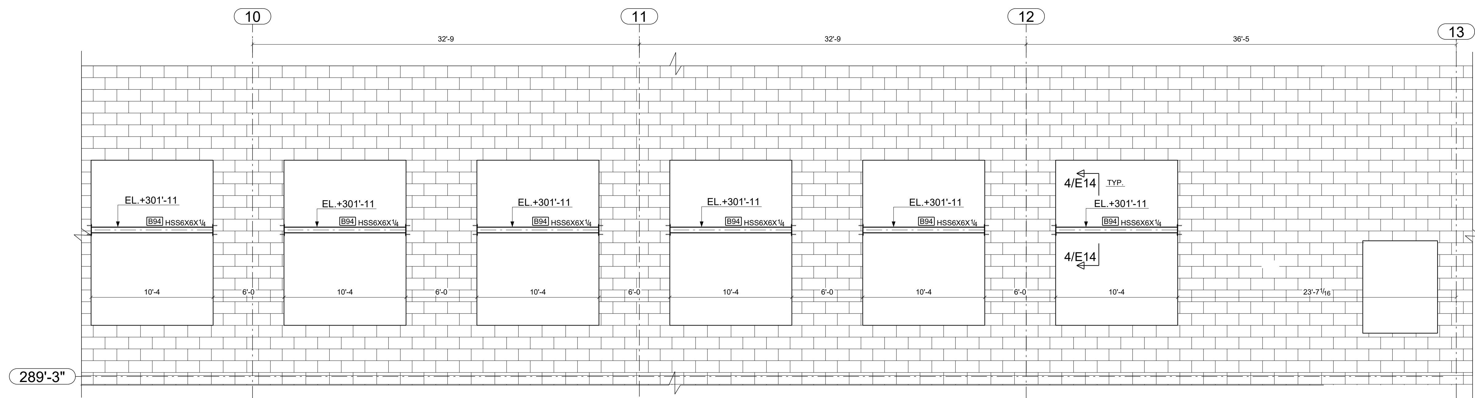
2 SOUTH WALL ELEVATION STEEL TUBE DETAILS SCALE: 1:60
