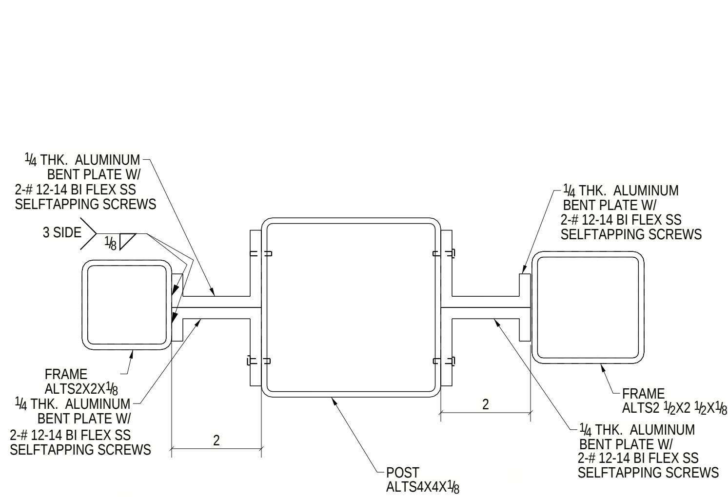
5 SECTION VIEW
