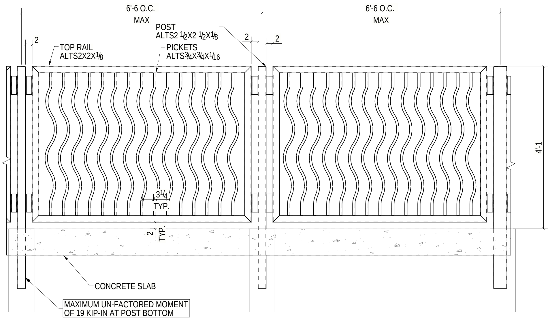
1 TYP. WAVY FENCE ELEVATION
