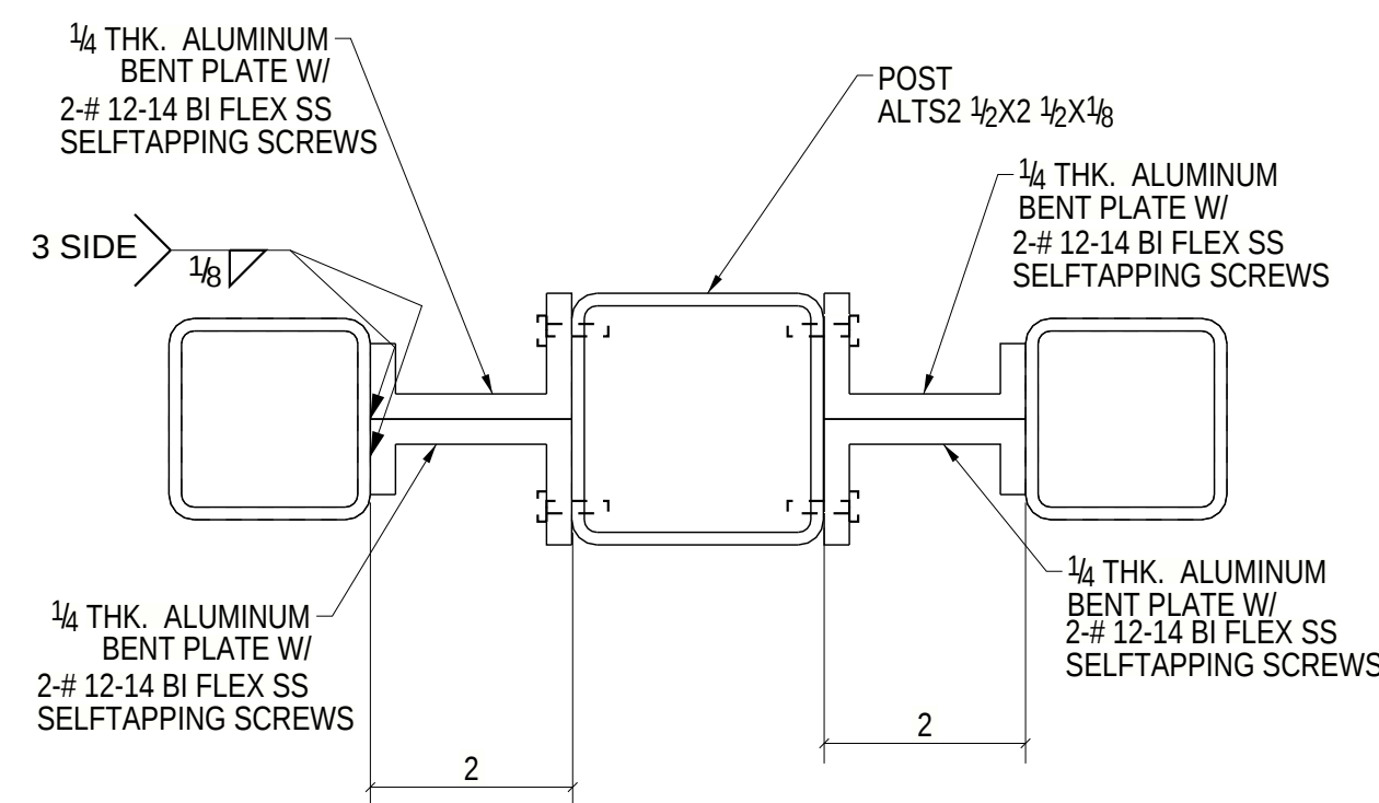
8 SECTION VIEW
