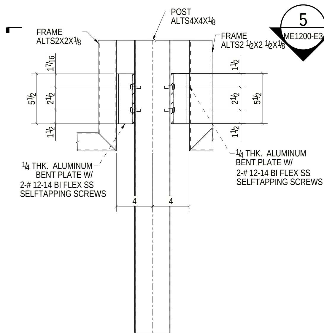
4 TYP. GATE FRAME TO POST CONN.
