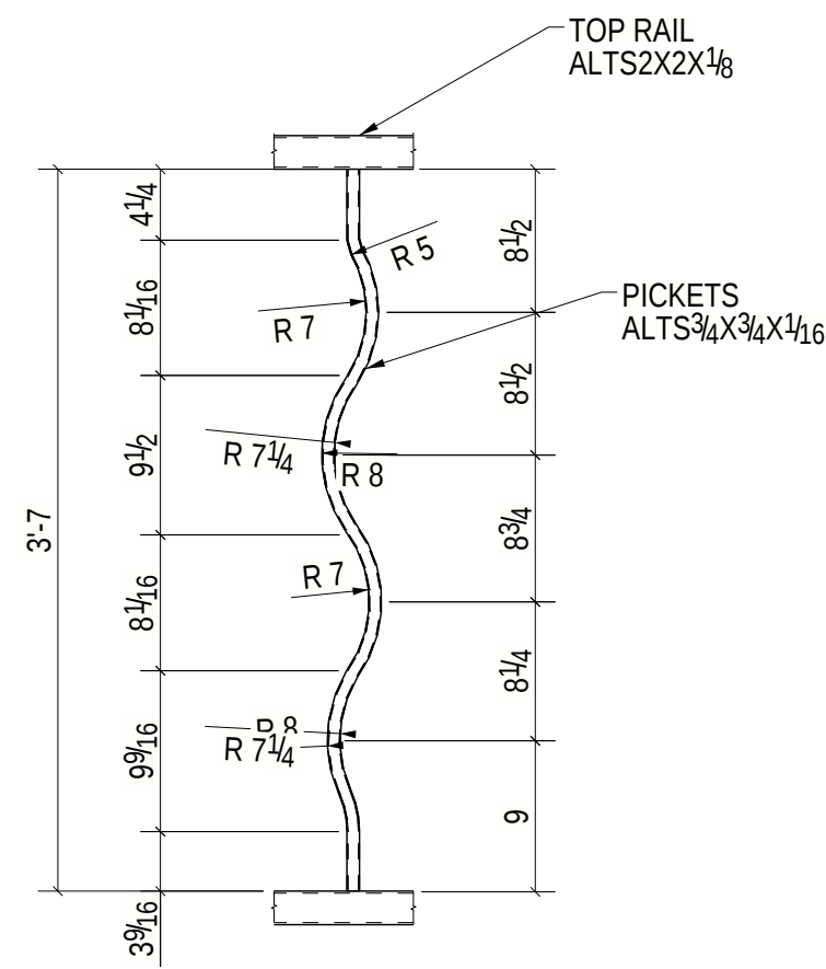
3 TYP. WAVY PICKET DETAIL
