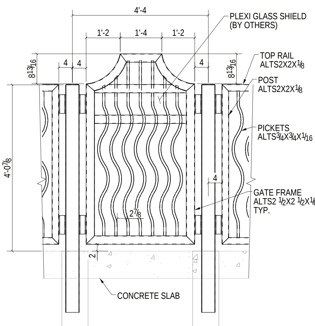
2 TYP. GATE ELEVATION
