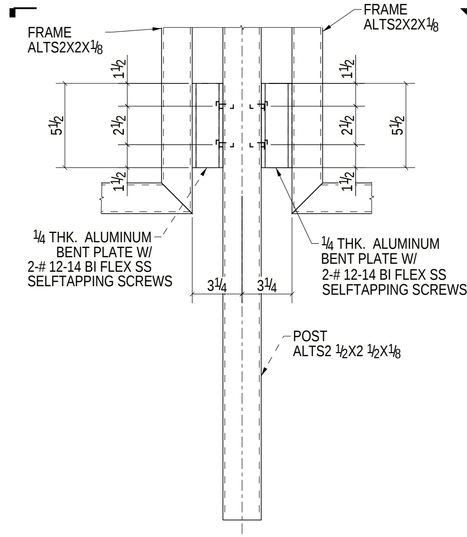
7 TYP. FENCE FRAME TO POST CONN.
