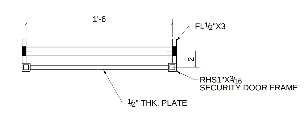
7 SECTION DETAIL
