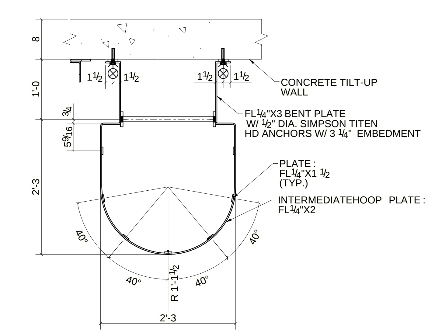
6 SECTION DETAIL
