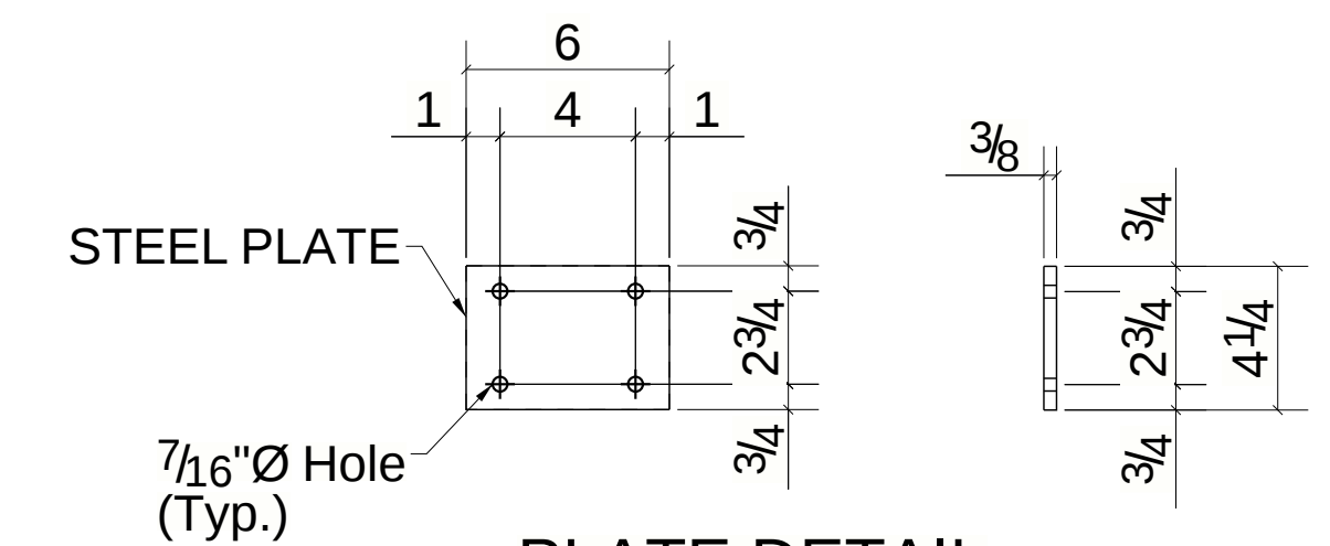
PLATE DETAIL
