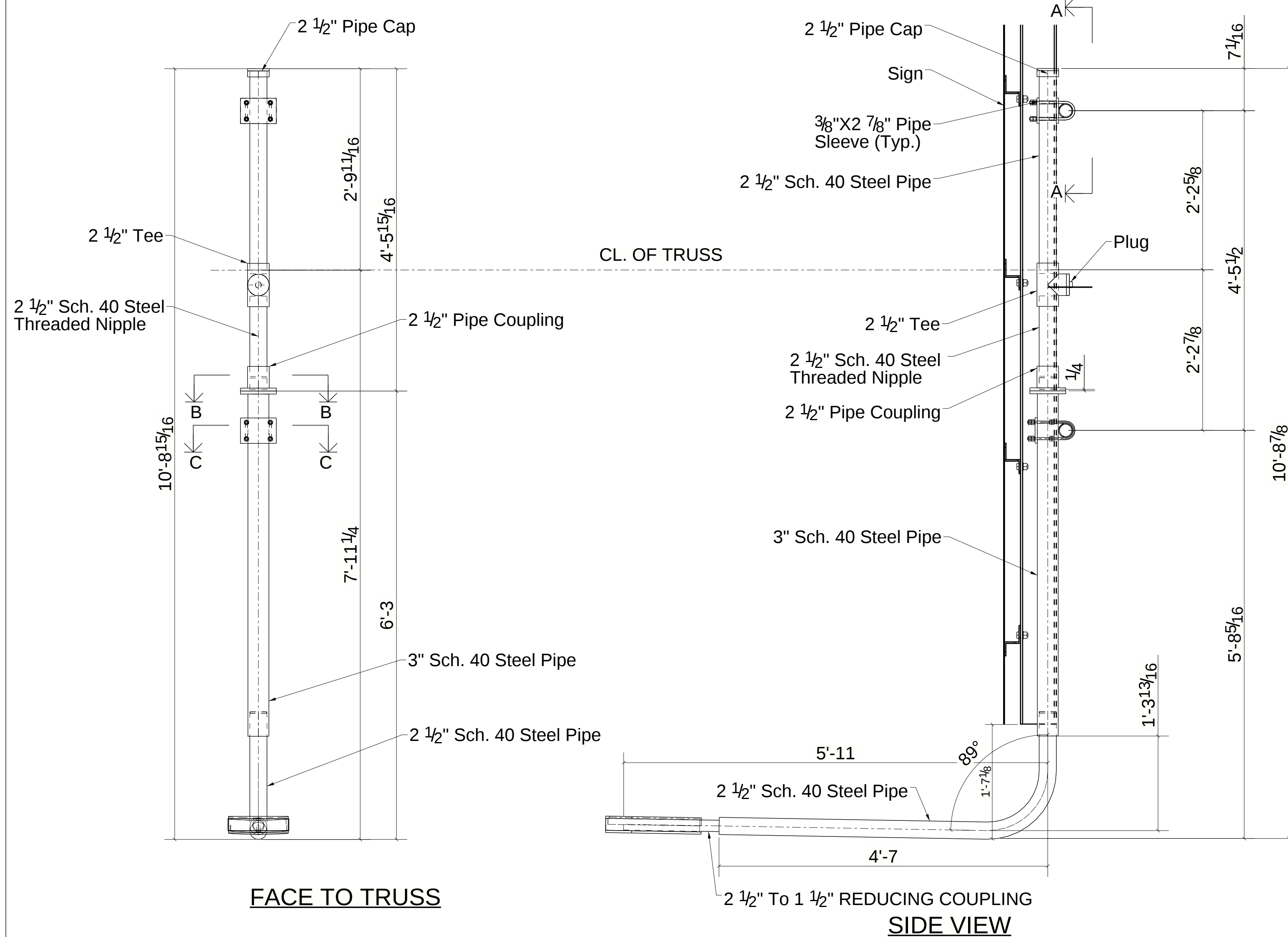
LUMINAR SUPPORT STRUCTURE
