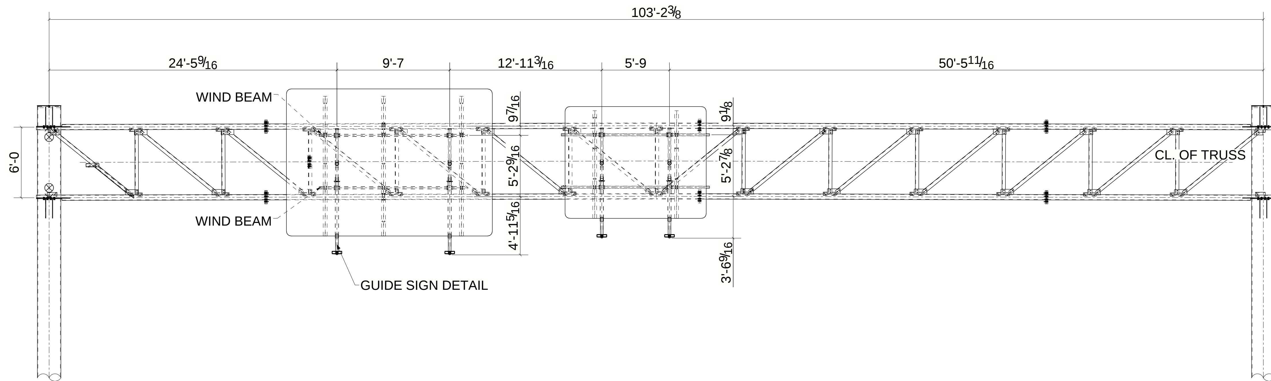
GUIDE SIGN DETAIL
