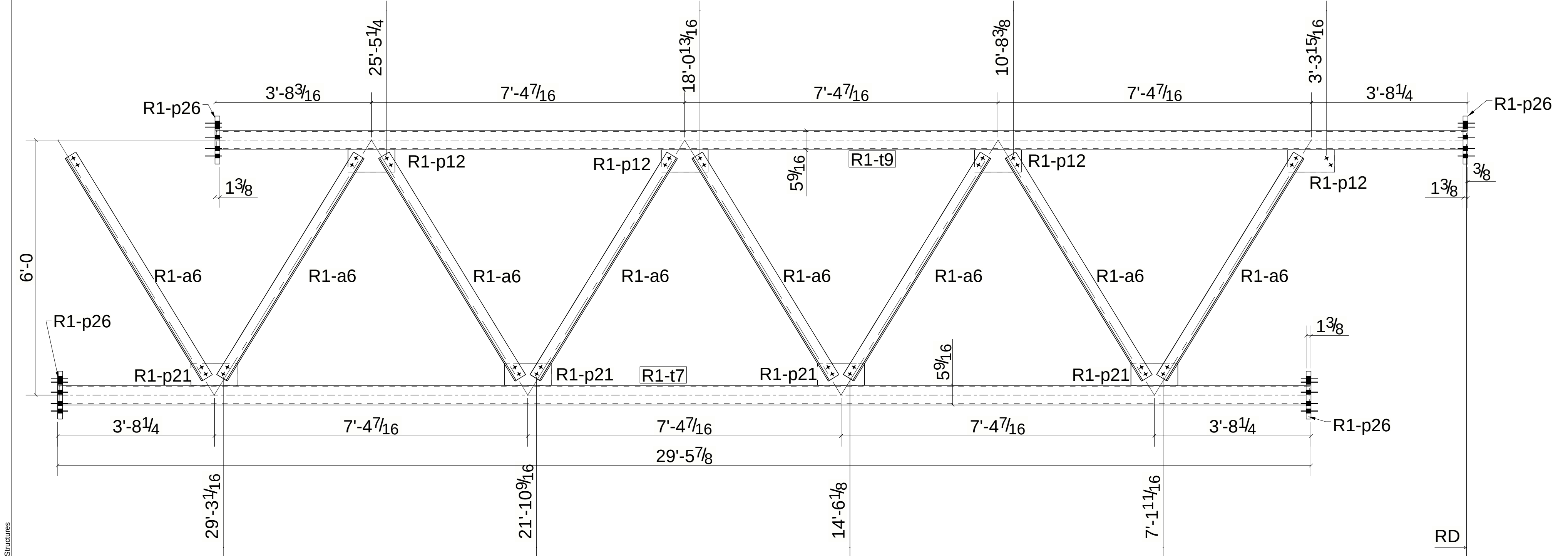
SPAN OTR-01 (SB) VIEW " F "
