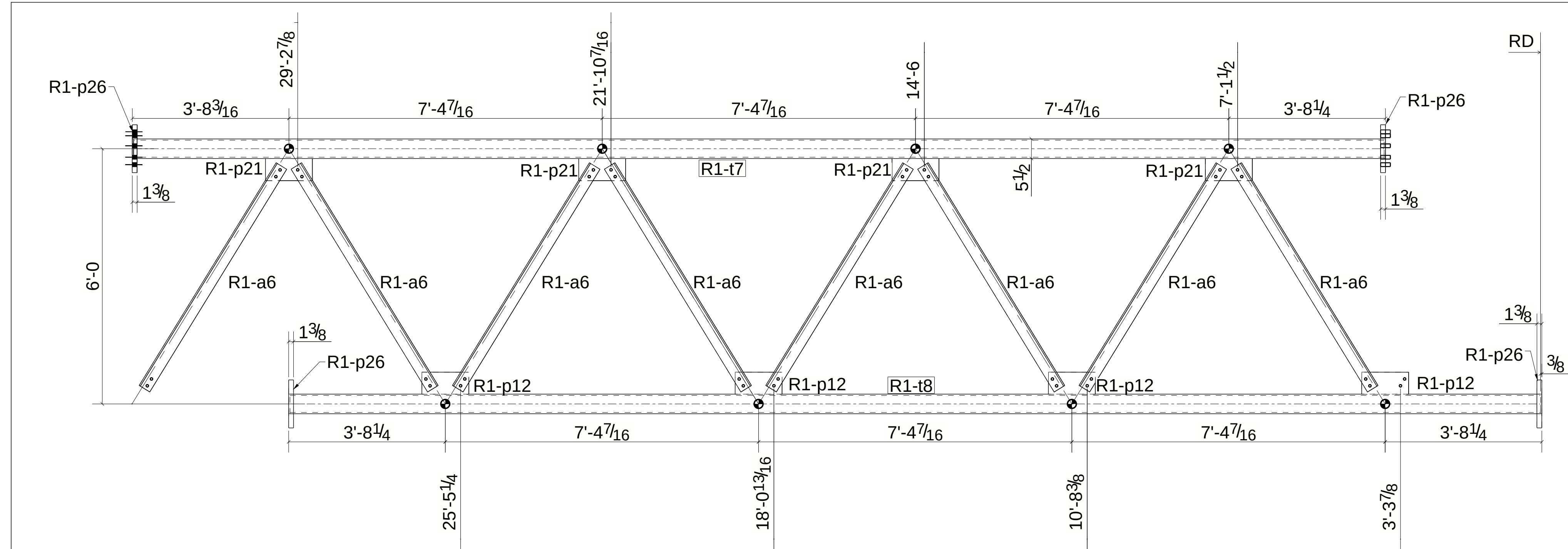
SPAN OTR-01 (SB) VIEW " E "
