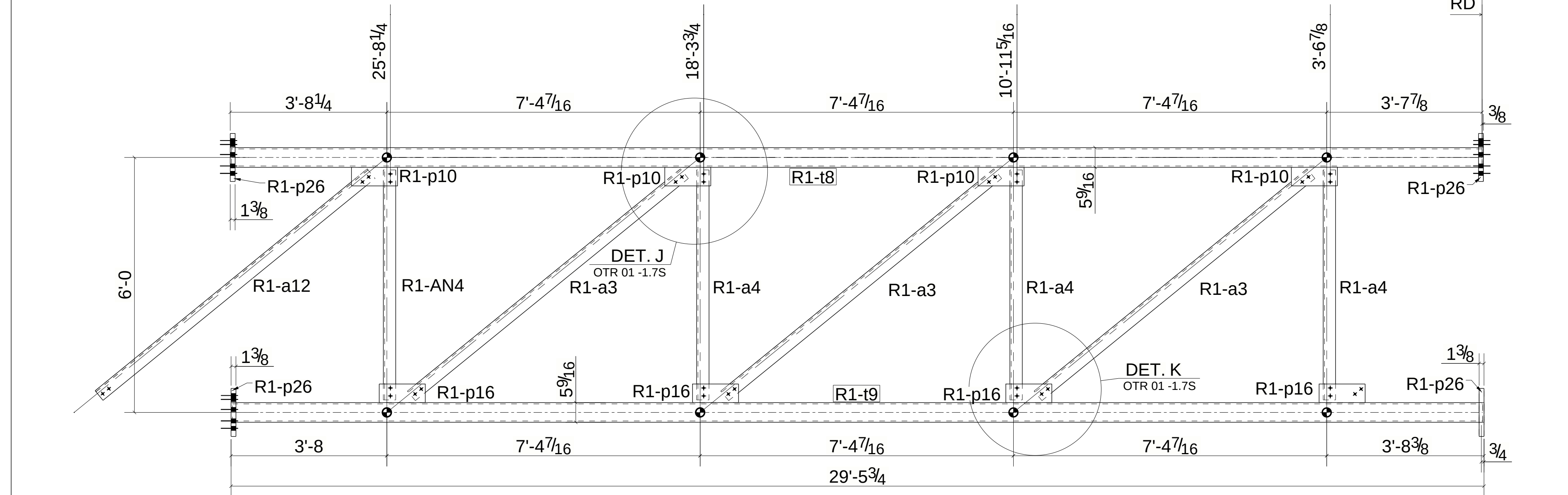
ELEVATION VIEW " B " SPAN OTR-01 (SB)
