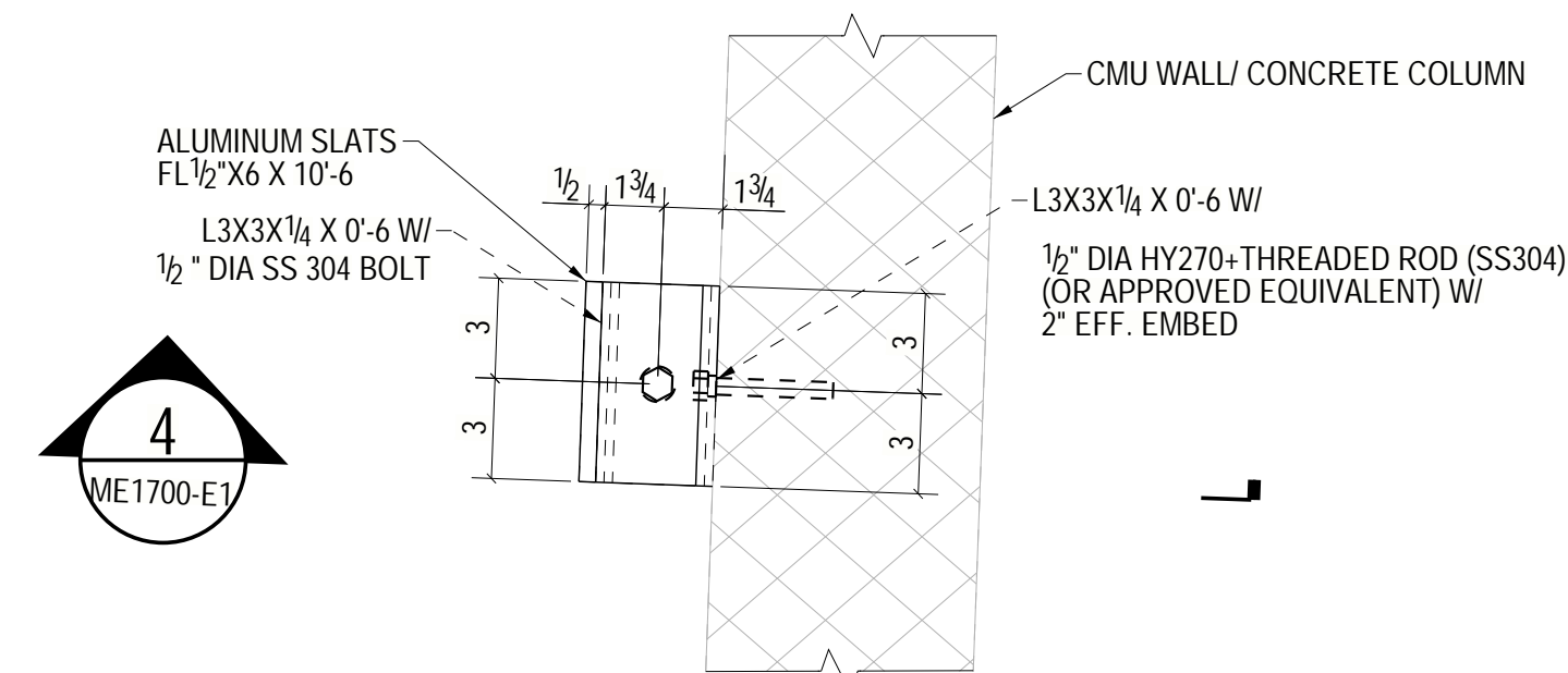
3 TYP. SLATS TO CMU WALL CONN. SCALE: 1:6
