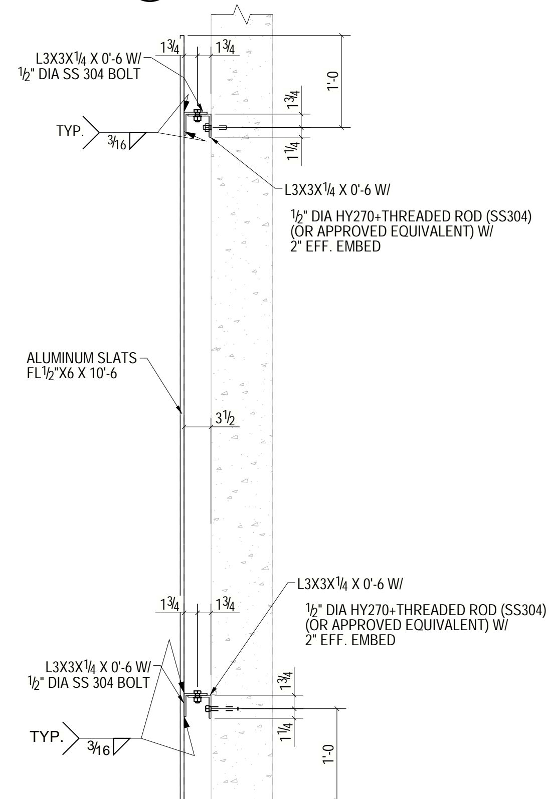
5 TYP. SLATS TO CONC. COLUMN CONN. SCALE: 1:6
