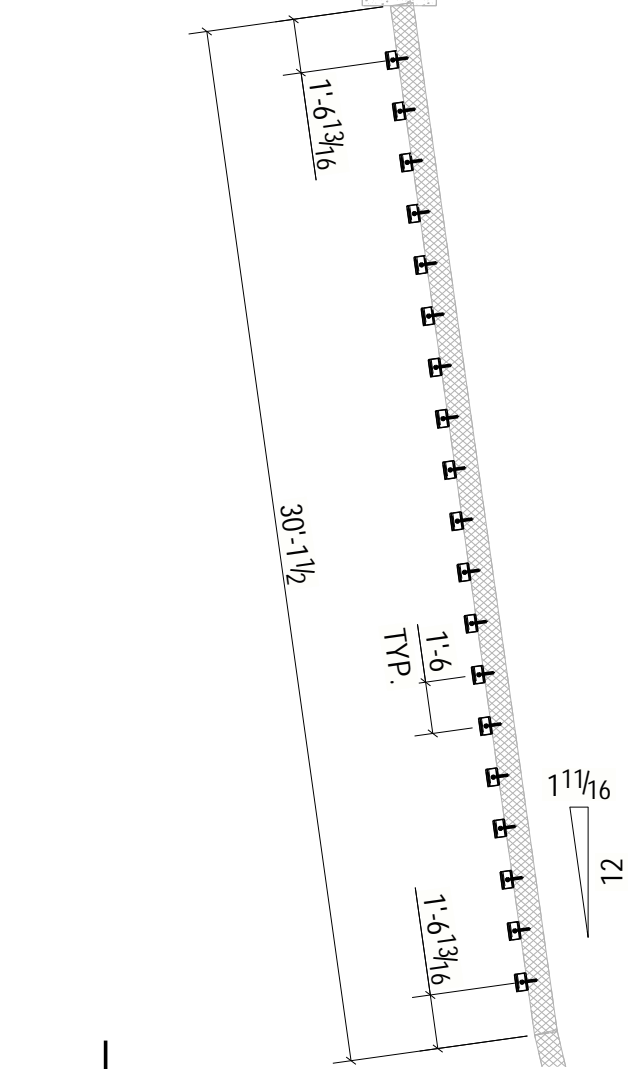
1 DECORATIVE ALUMINUM SLATS LAYOUT SCALE: 1:64
