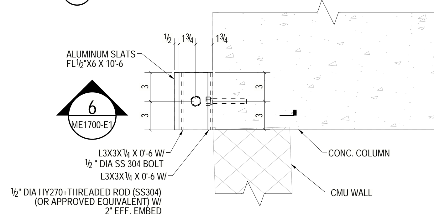
5 TYP. SLATS TO CONC. COLUMN CONN. SCALE: 1:6
